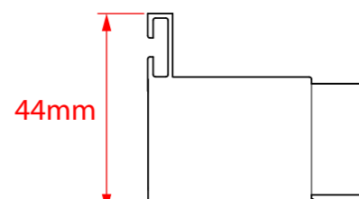
Door Panel fixing
